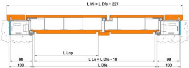
OBBLIGATORIO CON ESTETICA PANNELLO ESTERNO FAMILY BUGNE E MONOFRESATA MANDATORY WITH EXTERNAL PANEL AESTHETIC FAMILY EMBOSSED AND MONOMILLED
